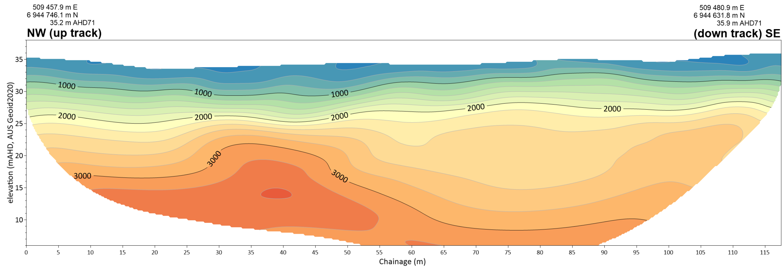
Seismic Line SR AU-GP 113
